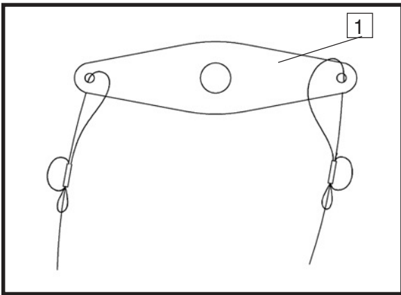
TAILWHEEL PUSHROD HORN INSTALLATION.
